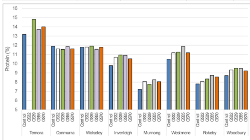
Figure 3. Effect of Nitrogen timing (combined rate and type) on grain protein across eight sites. Means followed by the same letter do not significantly differ ( p < 0.05 ).
