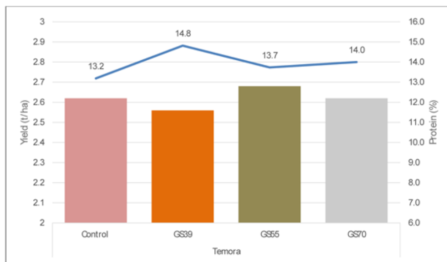
Figure 4. Effect of Nitrogen timing (combined type and rate) on grain yield (bars) and protein (line) - Temora. Means followed by the same letter do not significantly differ ( p < 0.05 ).
