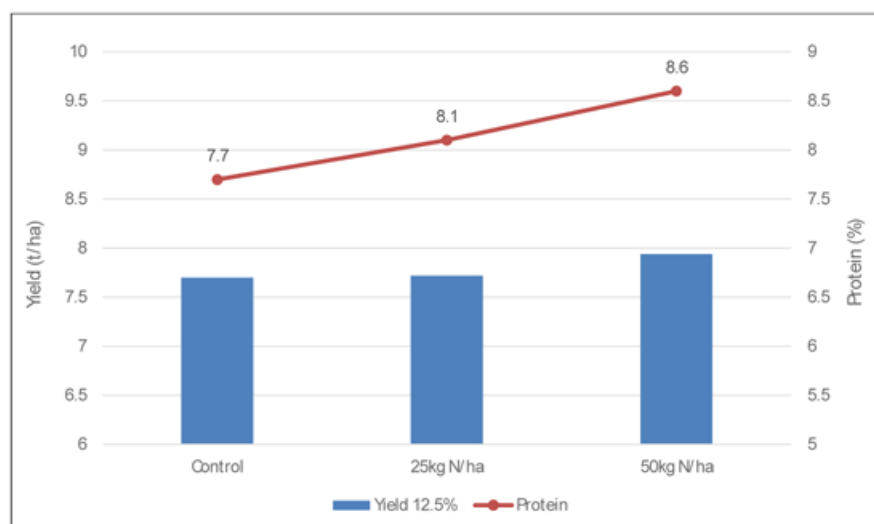
Figure 13. Effect of Nitrogen rate (combined type and timing) on grain yield (bars) and protein (line) - Rokeby. Means followed by the same letter do not significantly differ ( p < 0.05 ).
