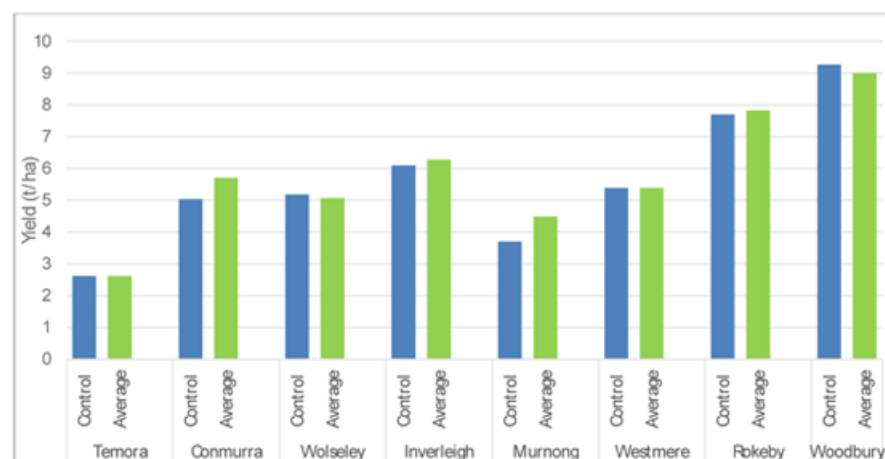
Figure 1. Effect of Nitrogen (combination of timing, rate and type) on grain yield across eight sites. Pairs of site means followed by the same letter do not significantly differ ( p < 0.05 ).
