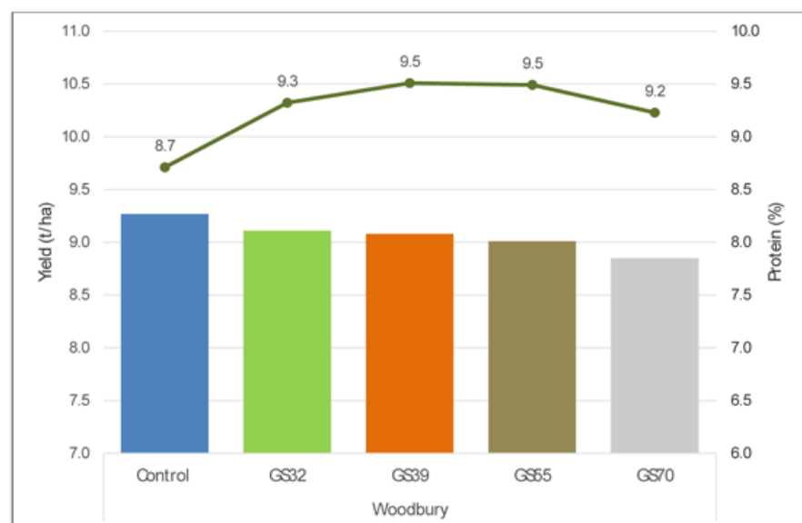
Figure 15. Effect of Nitrogen timing (combined type and rate) on grain yield (bars) and protein (line) - Woodbury. Means followed by the same letter do not significantly differ ( p < 0.05 ).
