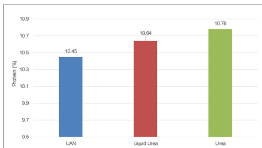
Figure 8. Effect of Nitrogen type (combined rate and timing) on grain protein - Inverleigh. Means followed by the same letter do not significantly differ ( p < 0.05 ).
