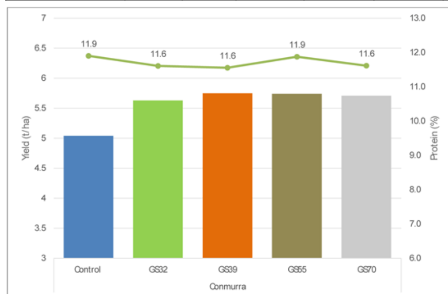
Figure 5. Effect of Nitrogen timing (combined type and rate) on grain yield (bars) and protein (line) - Conmurra. Means followed by the same letter do not significantly differ ( p < 0.05 ).
