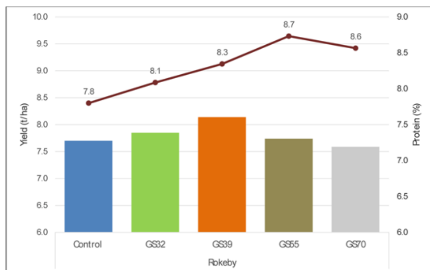
Figure 12. Effect of Nitrogen timing (combined type and rate) on grain yield (bars) and protein (line) - Rokeby. Means followed by the same letter do not significantly differ ( p < 0.05 ).
