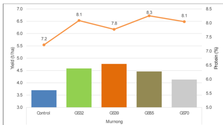
Figure 10. Effect of Nitrogen timing (combined type and rate) on grain yield (bars) and protein (line) - Murnong. Means followed by the same letter do not significantly differ ( p < 0.05 ).
