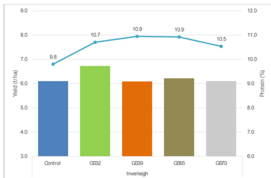
Figure 7. Effect of Nitrogen timing (combined type and rate) on grain yield (bars) and protein (line) - Inverleigh. Means followed by the same letter do not significantly differ ( p < 0.05 ).
