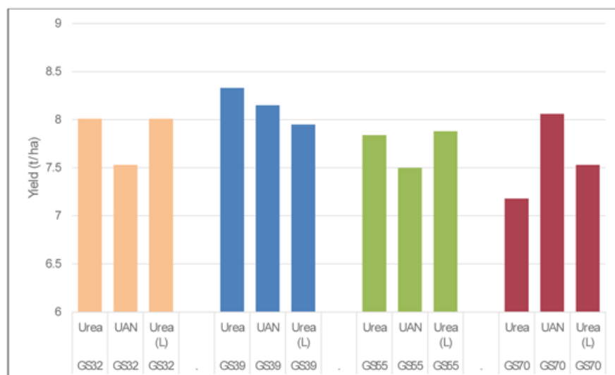
Figure 14. Effect of Nitrogen timing and type (combined rate) on grain yield - Rokeby. Means followed by the same letter do not significantly differ ( p < 0.05 ).
