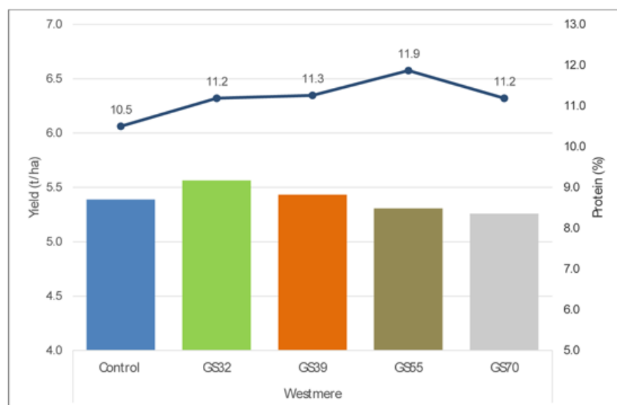
Figure 11. Effect of Nitrogen timing (combined type and rate) on grain yield (bars) and protein (line) - Westmere. Means followed by the same letter do not significantly differ ( p < 0.05 ).
